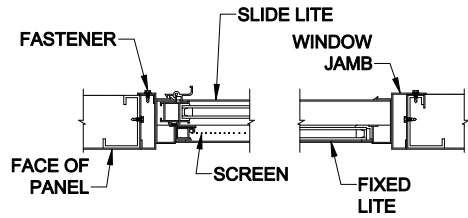
SECTION THRU WINDOW (TOP VIEW)
