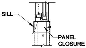
SECTION THRU WINDOW (SIDE VIEW)
