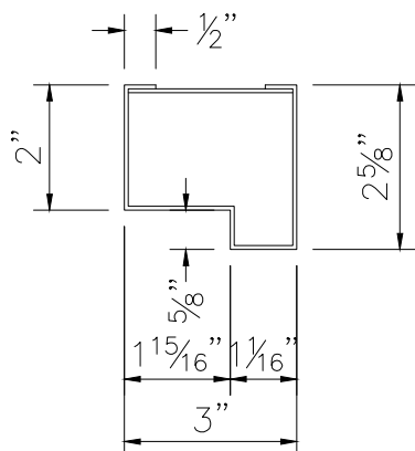
3" FRAME DIMENSIONS
