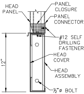
SECTION THRU HEAD
