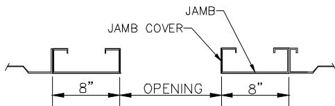
SECTION THRU JAMBS
