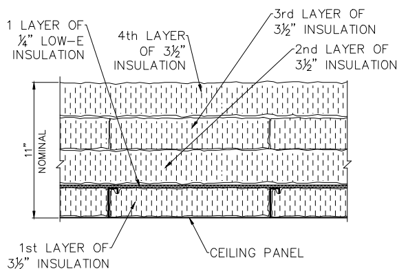
R49 INSULATION DETAIL
