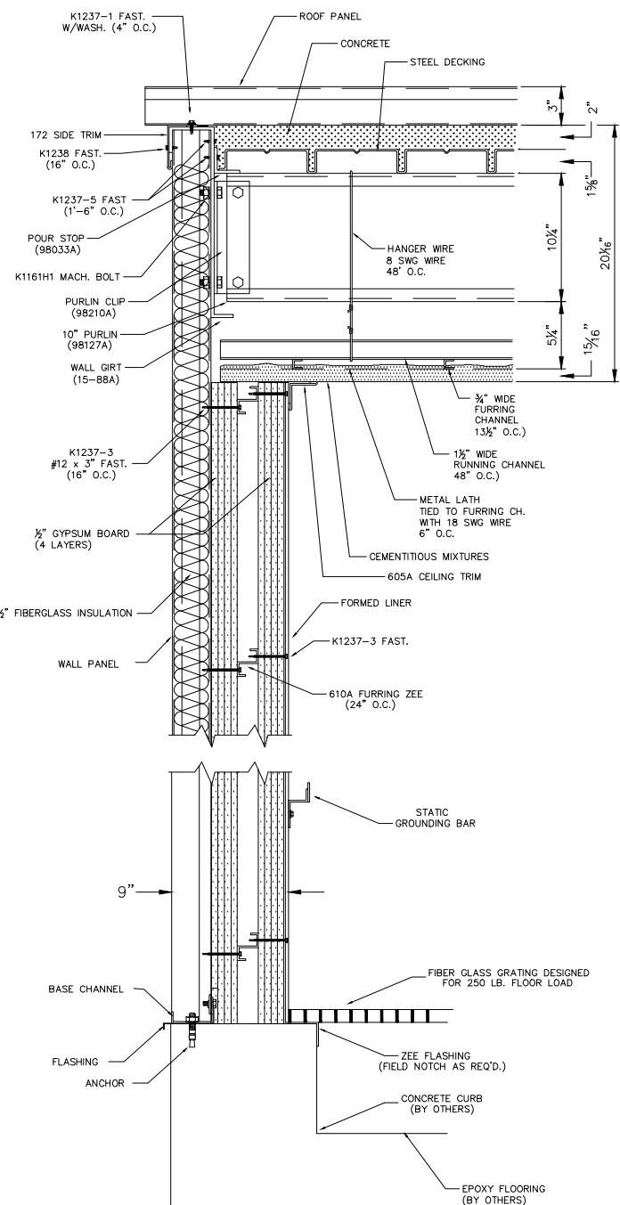
SECTION THRU SIDEWALL
