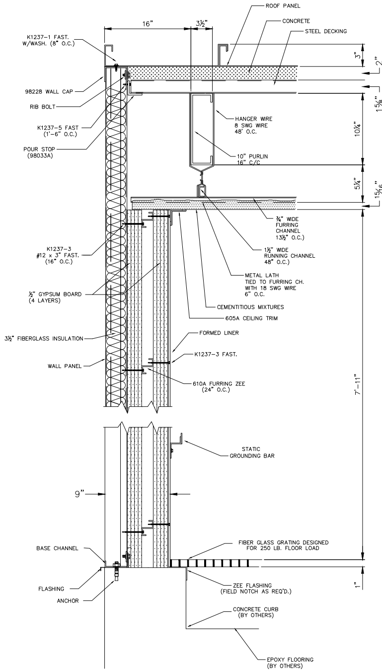
SECTION THRU ENDWALL
