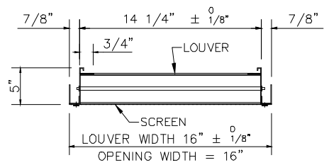
SECTION THRU LOUVER (TOP VIEW)
