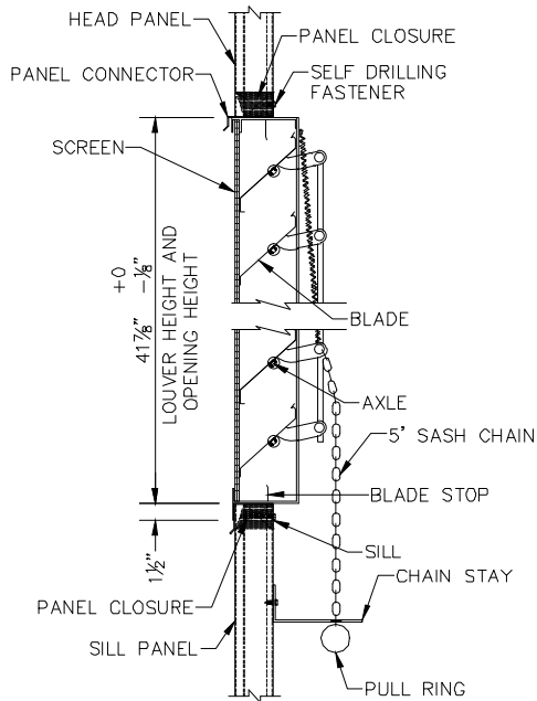
SECTION THRU LOUVER (SIDE VIEW)
