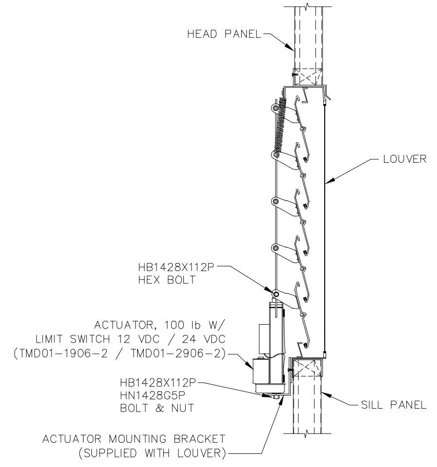
HORIZONTAL SECTION
