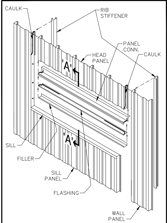
EXTERIOR ELEVATION
