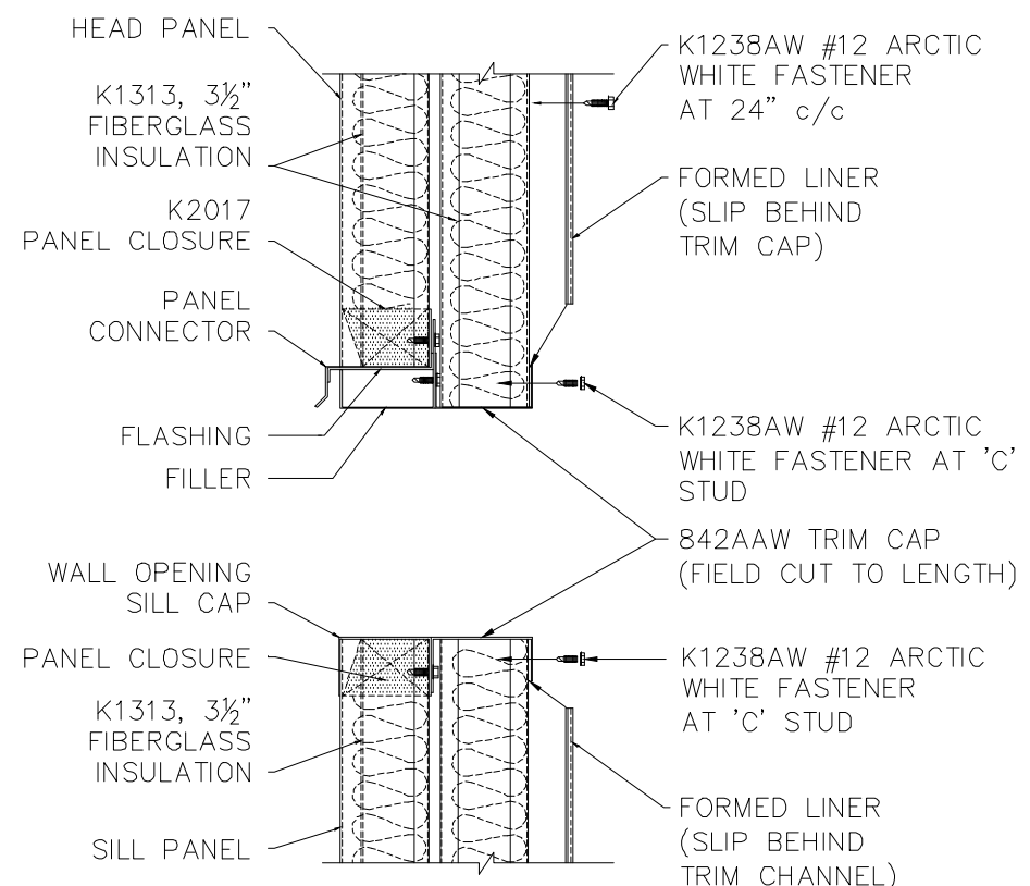
TRIM DETAIL AT WALL OPENING KIT (WINDOW SIMILAR)
