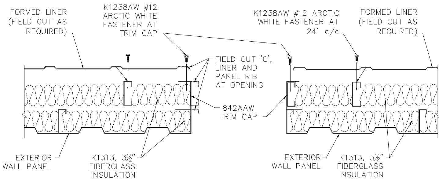
TRIM DETAIL AT WALL OPENING KIT (WINDOW SIMILAR)
