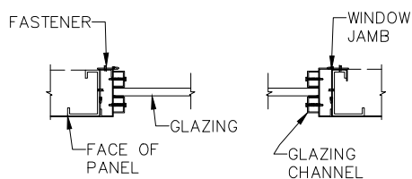
SECTION THRU WINDOW (TOP VIEW)
