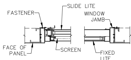
SECTION THRU WINDOW (TOP VIEW)
