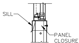
SECTION THRU WINDOW (SIDE VIEW)
