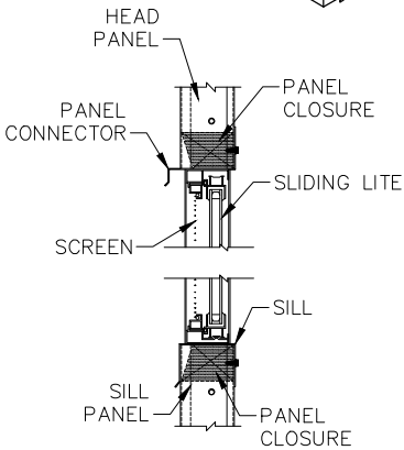
SECTION THRU WINDOW (SIDE VIEW)
